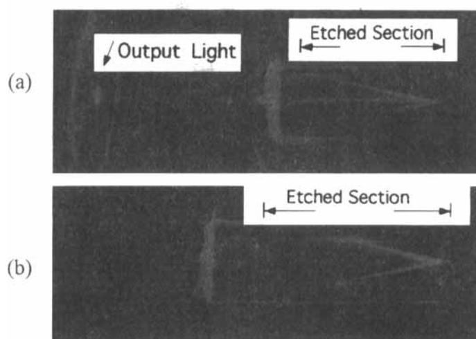
FIGURE 2 The effect of residual cladding thickness on lightwave propagation. (a) For b = 5 \mu\text{m} , the light leaked out in propagating through the etched section of the fiber, but output from the fiber end continued. (b) For b = 3 \mu\text{m} , the light decayed dramatically and disappeared completely from the output. (See Color Plate XVIII).
